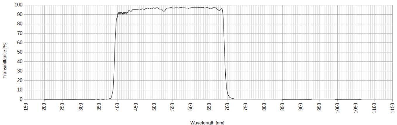
Transmittance chart
